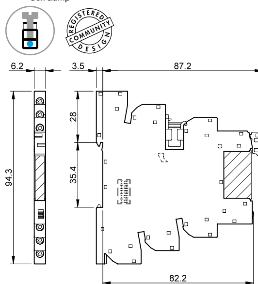
Types 39.80 39.81 Box clamp
