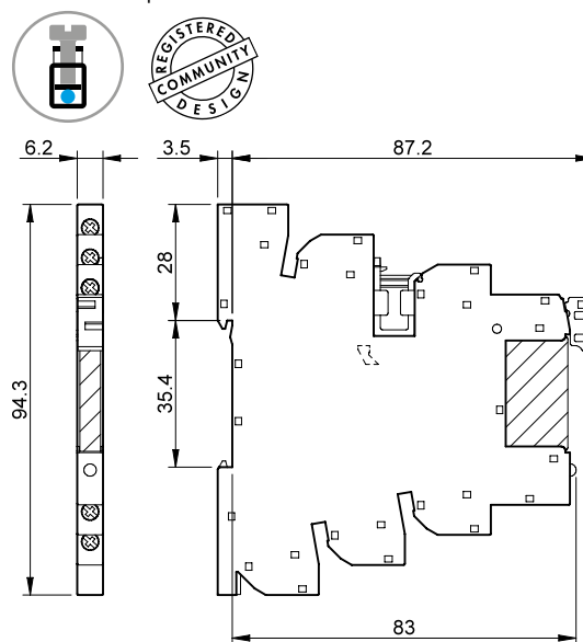
Types 39.30/39.30.3 39.31/39.31.3 Box clamp
