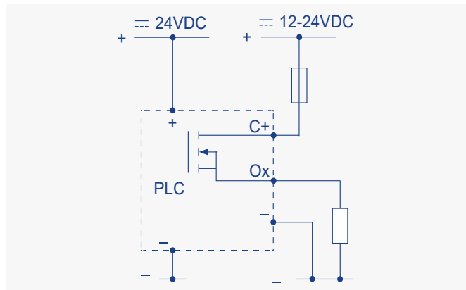
Electronic Diagram
