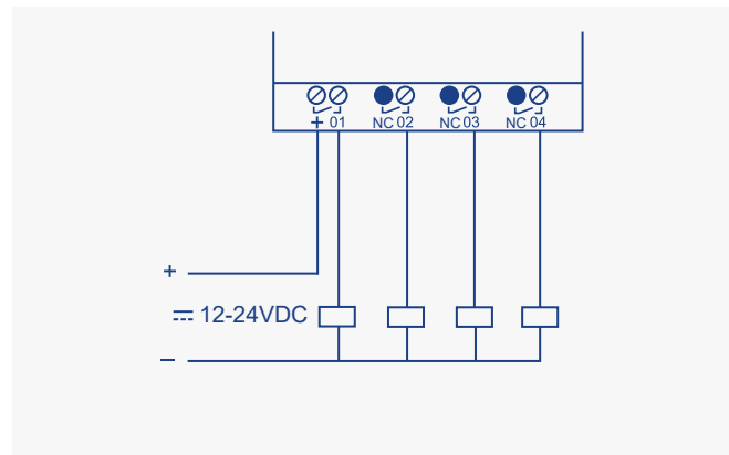
Wiring Diagram
