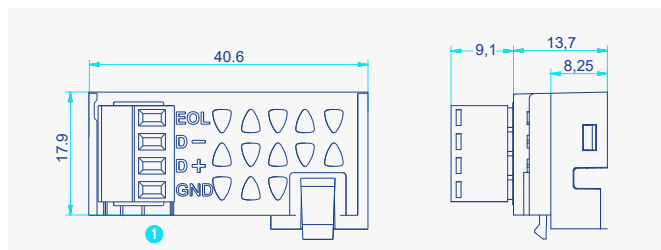
1 Connection terminals
